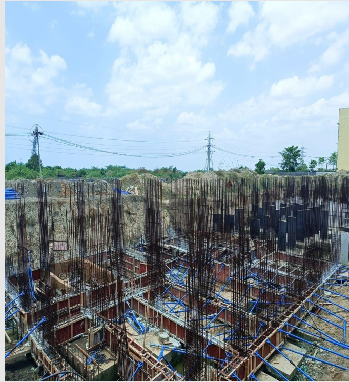
UG sump plinth beam concrete completed. waterproofing dimple board protection sheet works in progress
