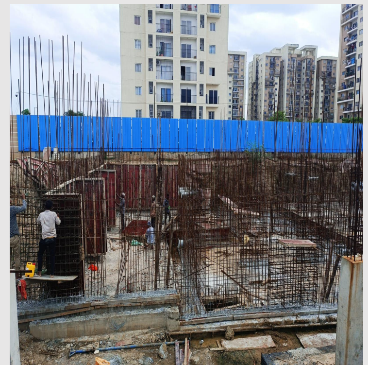
UG Sump pump room and fire sump wall starter concrete completed and pedal flange fixing works and sump wall shuttering works in progress
